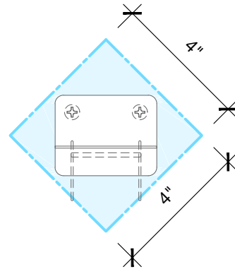
CLADDING ATTACHMENT DETAIL CA-1: TYPICAL CLADDING ATTACHMENT SIGA WIGLUV® 3.9" PATCH ELEVATION
